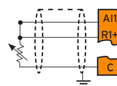
RTD In
