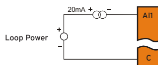
20mA Analog In - Not Self Powered
